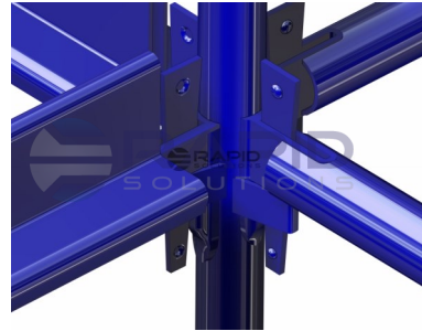
KWIKSTAGE SYSTEM
