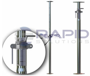
ACROW PROPS
