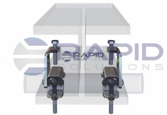
GRAVLOCK GIRDER COUPLER
