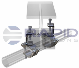
GRAVLOCK SWIVEL COUPLER
