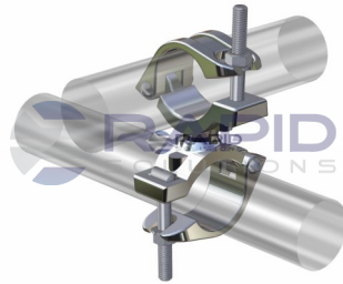
SWIVEL COUPLER
